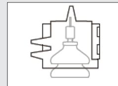
Figure 2: Cover style wildlife protector shown installed on transformer bushing
