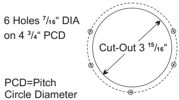
CUT-OUT DETAILS
